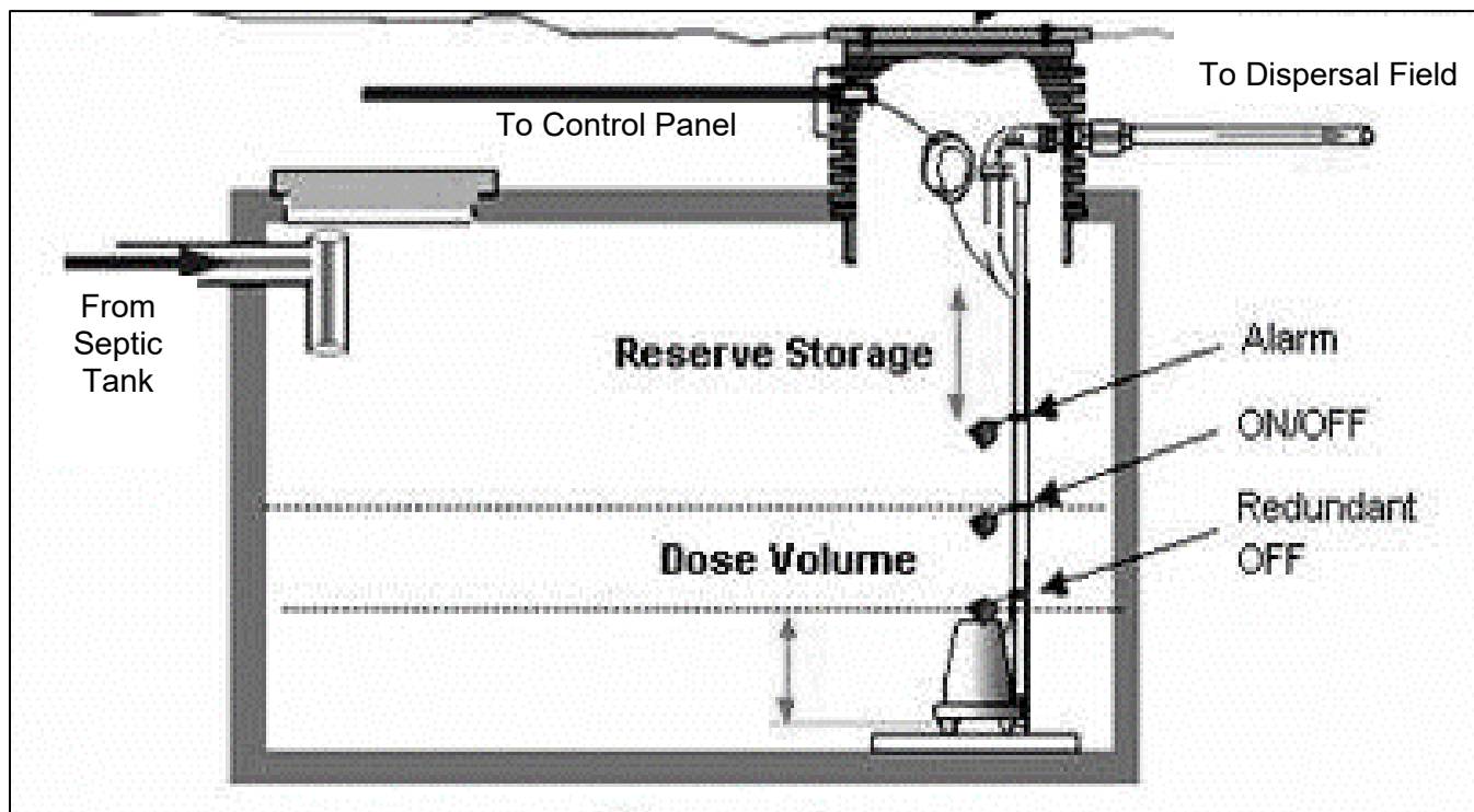
Figure 2-Typical Pump Tank
