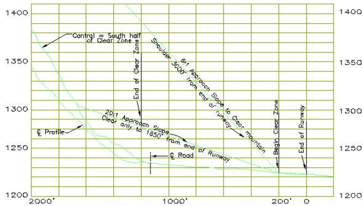
Profile - Approach to Runway 10 Scales: Horiz: 1"=200' Vert: 1"=30'
