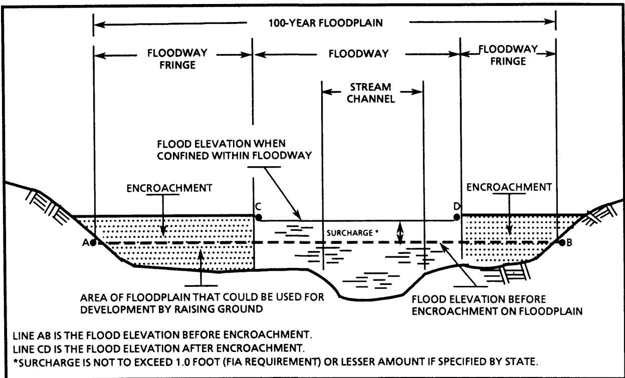
Figure 8. Floodway Schematic
