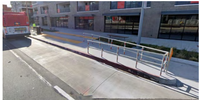
Photo 12: Example of sidewalk level crossing for pedestrians where bicycles ramp up and then down through bus stop. (Long Beach, California)
