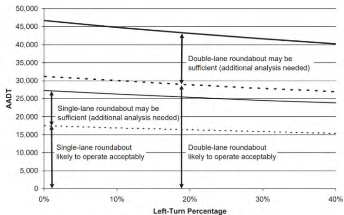
Figure 10: Potential Roundabout Capacity Based on Volumes and Geometrics (Source: FHWA, 2010)
