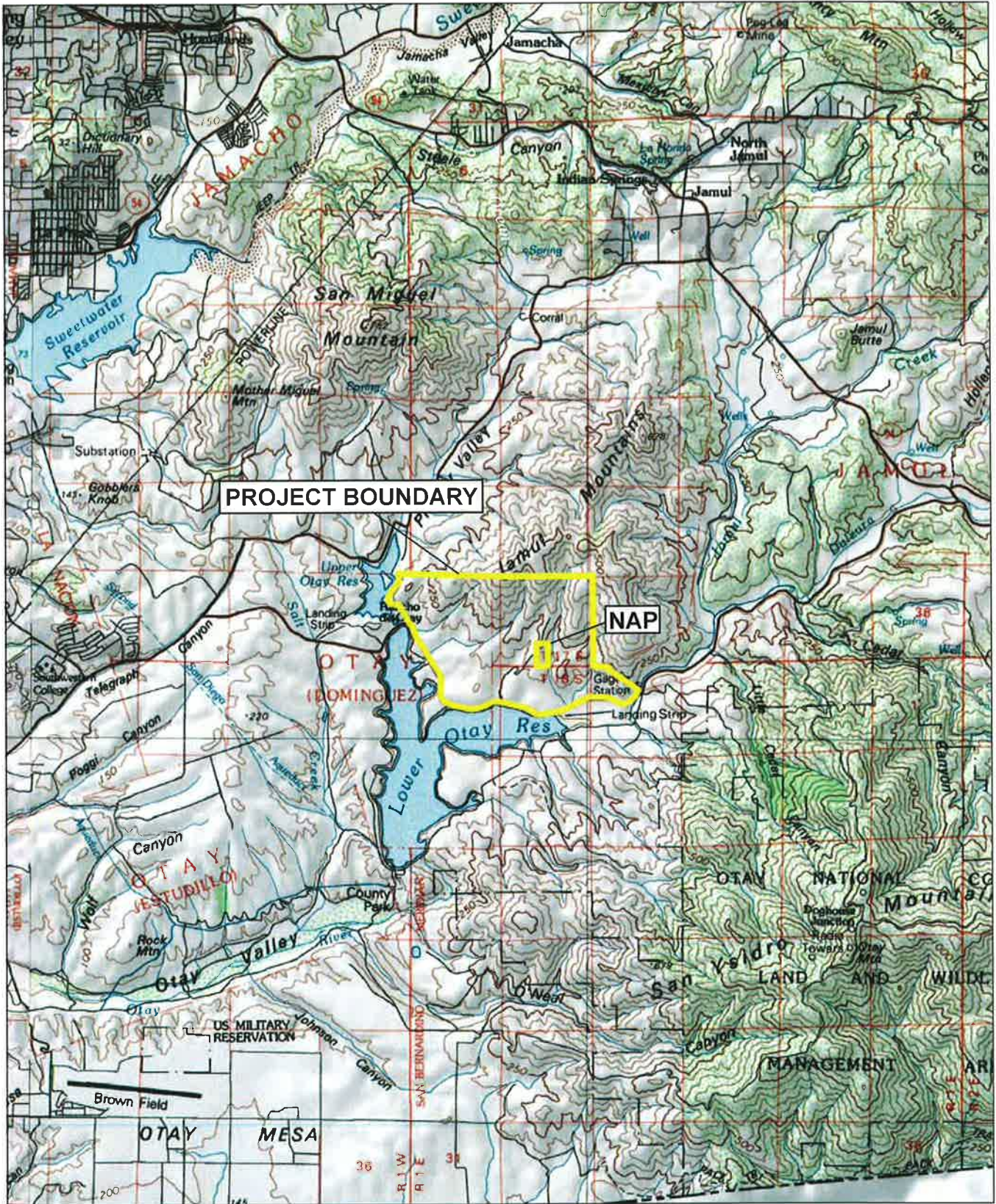
Figure 1.0-14 USGS Quadrangle
