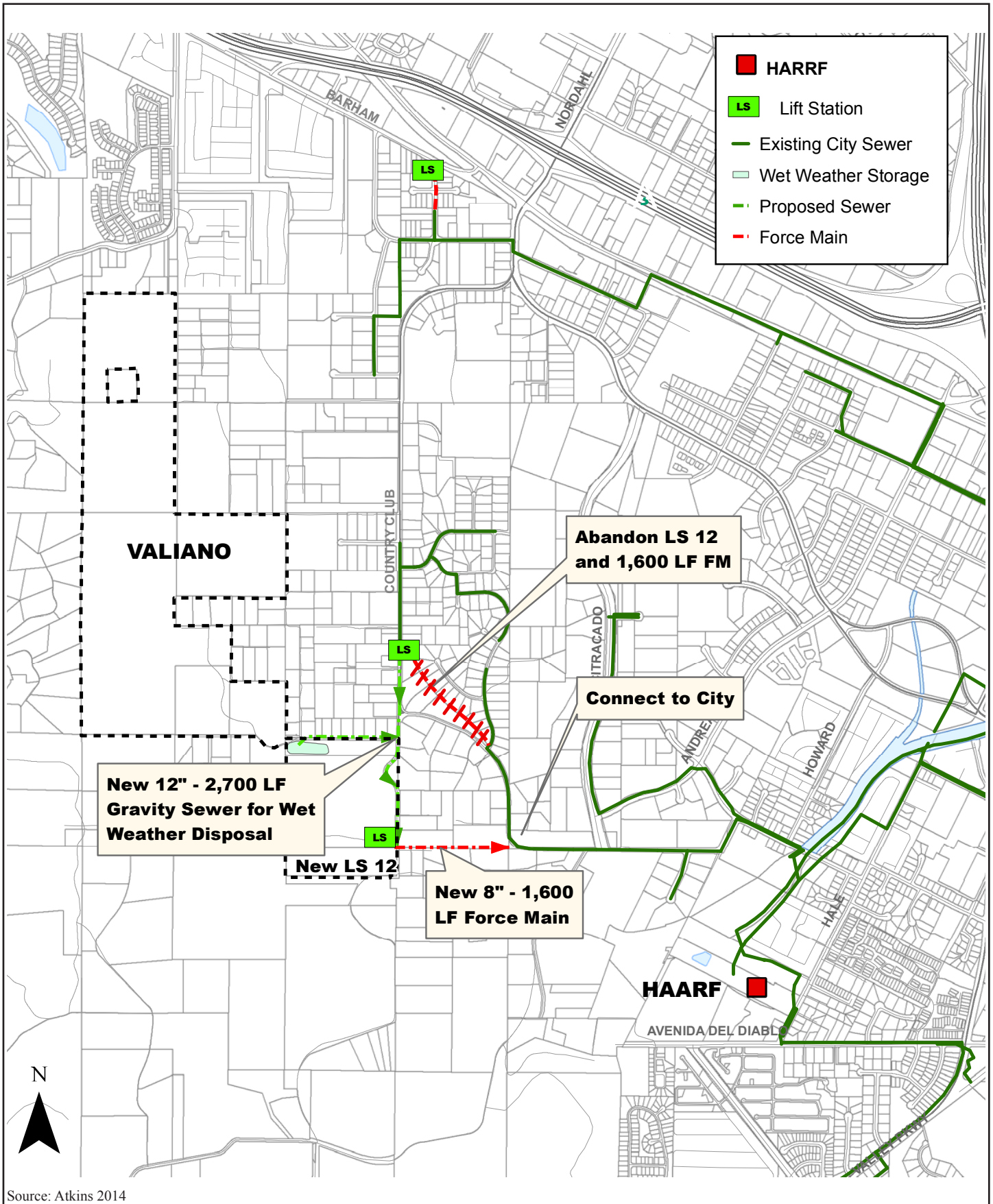
Connection to City of Escondido Hale Avenue Resource Recovery Facility VALIANO Figure 4-3
