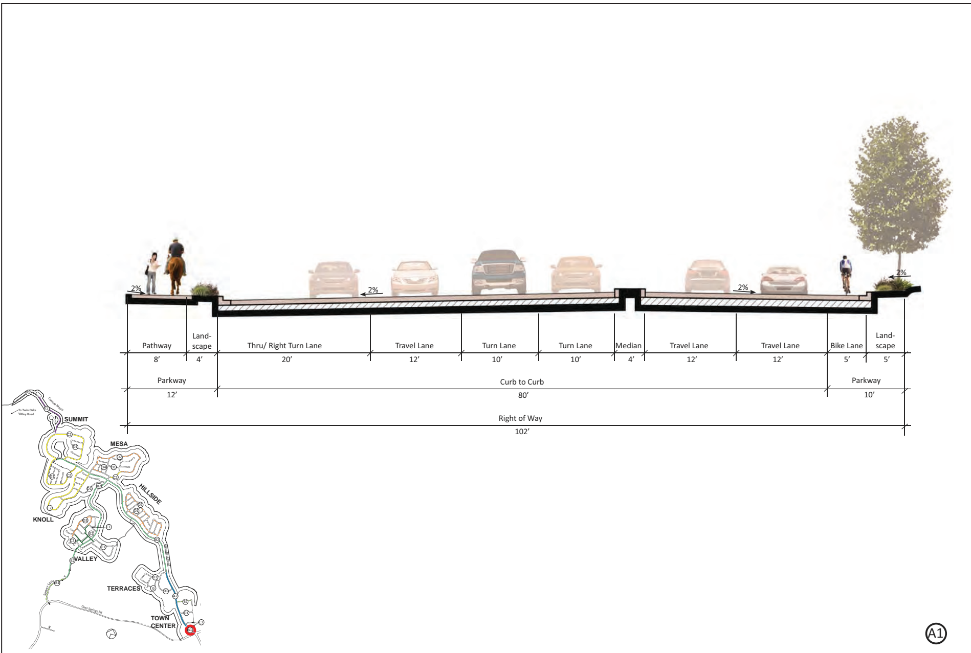
FIGURE 15 Public Modified Boulevard with Raised Median
