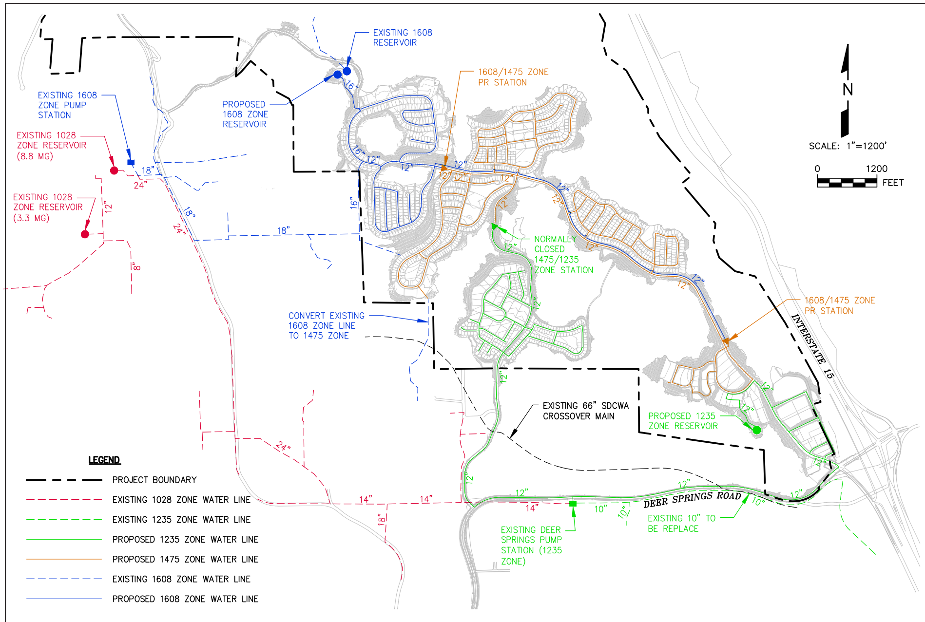
FIGURE 30 Water Supply
