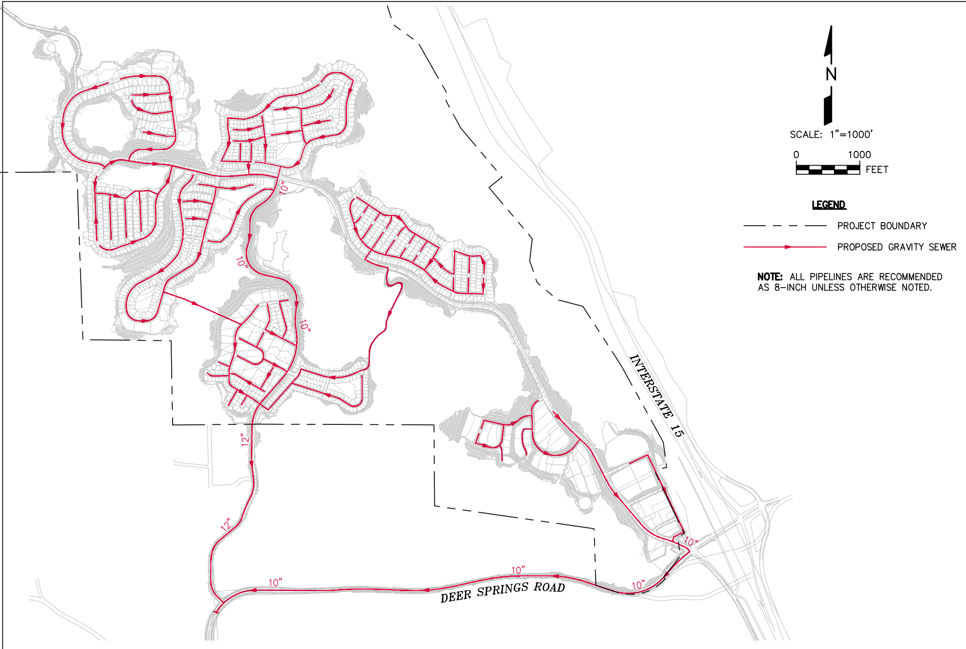
FIGURE 31 Sewer Collection Supply Newland Sierra Specific Plan
